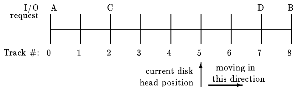
Fig. 2. Disk scheduling example.
