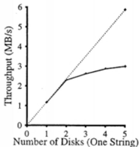
(a) Varying Disks Per String
