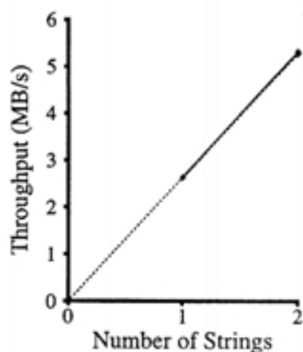
(b) Varying Strings Per Controller
