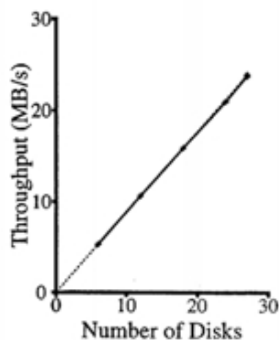
(b) Varying Strings Per Controller
