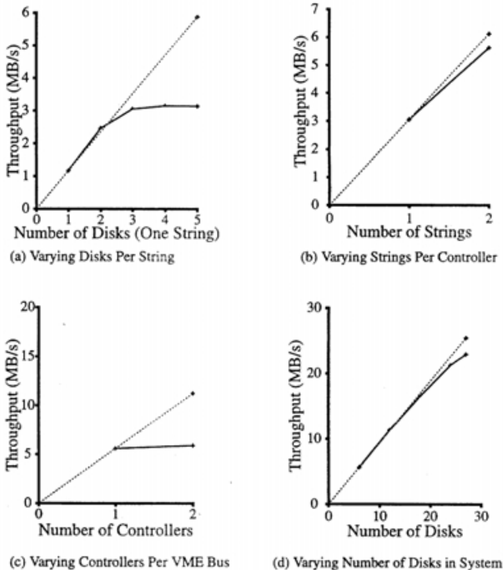
Figure 6. Disk Write Performance. This figure shows how disk write performance scales with increasing numbers of disks. Figure (a) uses one string on one Interphase Cougar and varies the number of disks from 1 to 5. Figure (b) fixes the number of disks per string at three and varies the number of strings per Cougar from 1 to 2. Figure (c) varies the number of Cougars per VME bus from 1 to 2, fixing the number of disks per string at three and the number of strings per Cougar at two. Figure (d) varies the number of VME busses attached to the XBUS card from one to four, fixing the number of disks per string at three, the number of strings per Cougar at two, and the number of Cougars per VME bus at one. These tests measure raw disk write performance—the disk array is configured without redundancy. Dotted lines show linear speedup.
