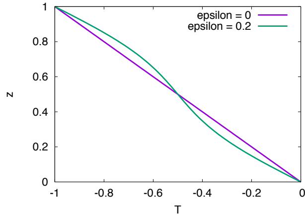
Figure 5.7: Mean temperature profile for the background state ( \epsilon = 0 ) and for the weakly nonlinear steady state solution with \epsilon = 0.2 .
