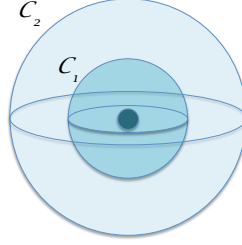
Figure 2.18: Spherical surfaces around the spherical loudspeaker. The energy flux through each spherical shell has to be the same.
