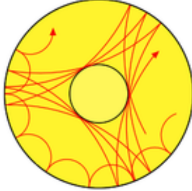
Figure 2.15: Examples of ray paths of waves in a star or planets, after several bounces/refractions. Image from Wikipedia.
