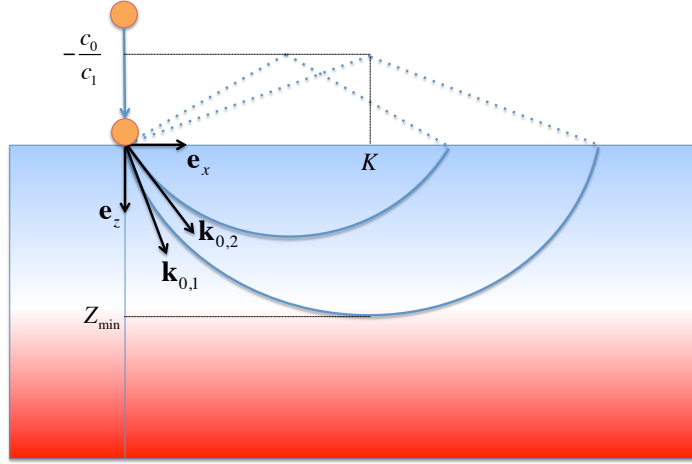
Figure 2.14: Examples of ray paths of waves emitted by a comet falling on the surface of a star or planet. Two representatives ray paths are shown. The initial wave vector \mathbf{k}_{0,i} of the two waves has the same amplitude but \mathbf{k}_{0,1} has a smaller k_{x0} and a larger k_{z0} while \mathbf{k}_{0,2} has a larger k_{x0} and a smaller k_{z0} . In both cases, the ray paths are arcs of circles, and the centers of these circles are given in the text.
