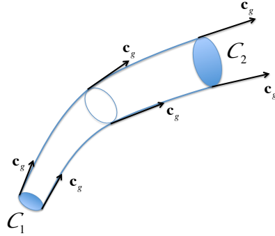
Figure 2.17: Example of a ray tube.
