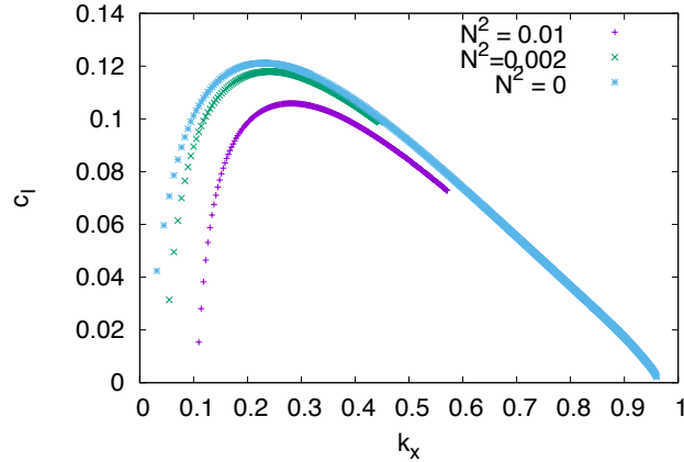
Figure 6.2: Imaginary part of c for the varicose mode of the Bickley jet for increasing values of N^2 .
